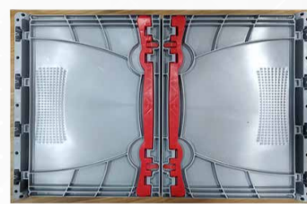
FOLDED VIEW
